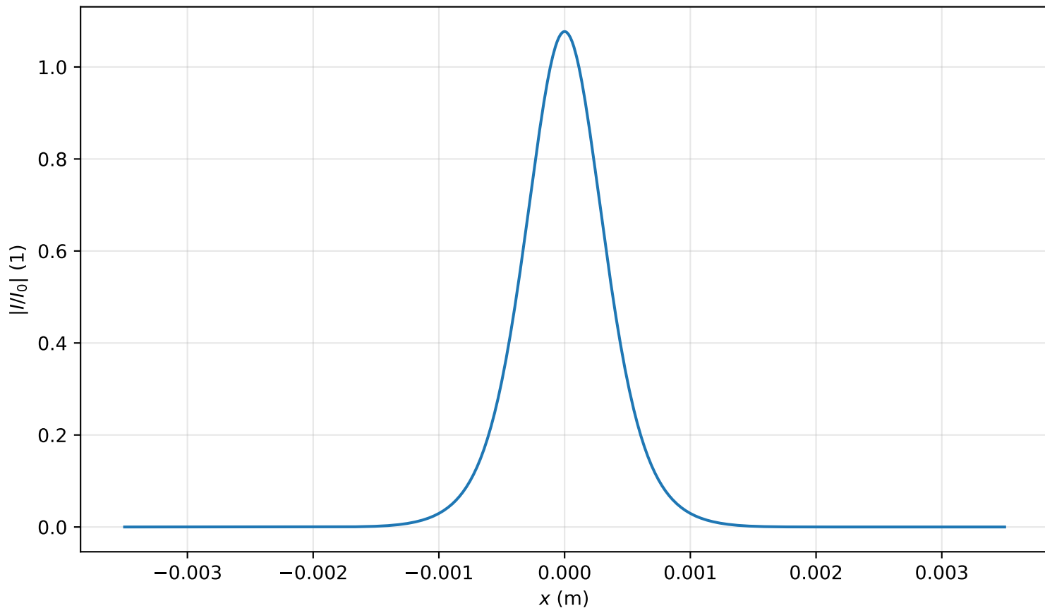
Intensity profile I(x, y = 0, z = 1.433m)/I_0 , P_{in}=0.6P_{cr} , artificial time
